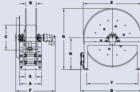
Series SPB800 - Rollformed Frame
